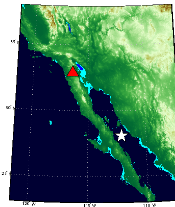
The location of station AZ_MONP is shown by the red triangle; the white star depicts the location on the surface directly above the earthquake.
