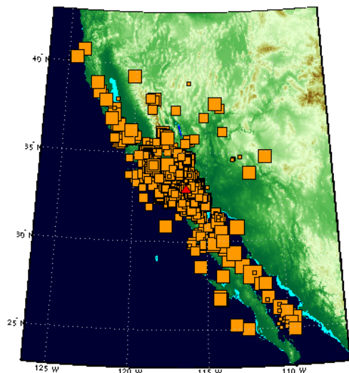
Regional events detected by station AZ_MONP. The size of the orange squares is proportional to the magnitude of the event. Station AZ_MONP is shown by the red triangle.
