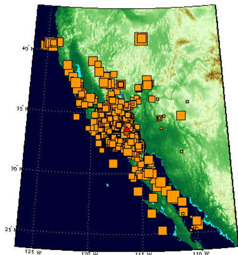
Regional events detected by station AZ_PFO. The size of the orange squares is proportional to the magnitude of the event. Station AZ_PFO is shown by the red triangle.
