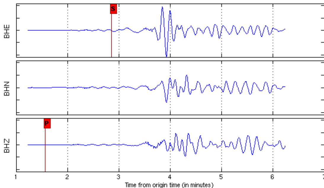
Three components recorded from the magnitude 6.2 regional event detected by station AZ_PFO on 1/04/2006 ( 8:32:31.570 UTC ). This occurred approximately 743 km from the station. The first seismic waves (P waves) arrived at this station 94.1 seconds after the event occurred.
