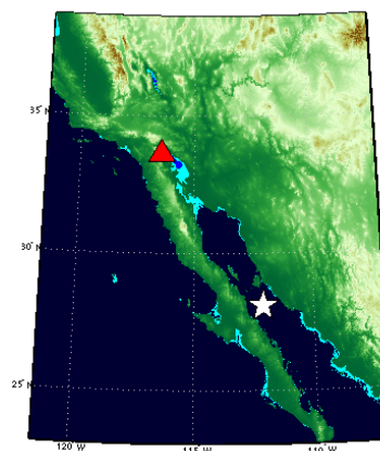
The location of station AZ_PFO is shown by the red triangle; the white star depicts the location on the surface directly above the earthquake.
